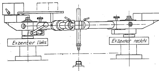
principle diagram of lever arm system
